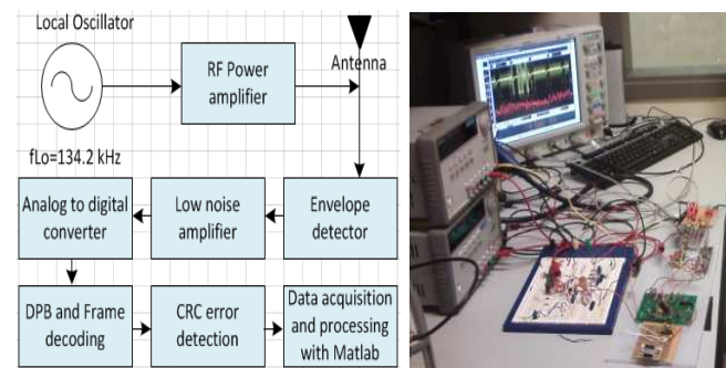
Fig. 6. Architecture of RFID base station (Left) and Test bed of an RFID system (Right)
